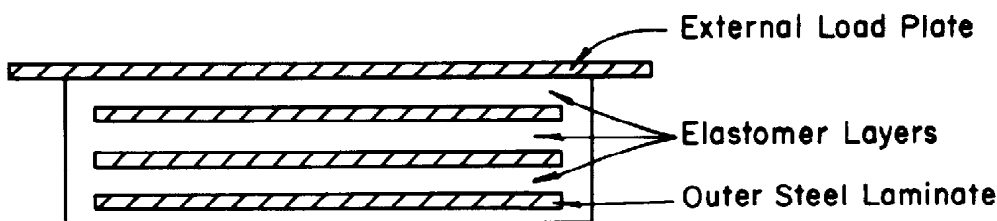
STEEL-LAMINATED ELASTOMERIC BEARING (With One External Load Plate)
