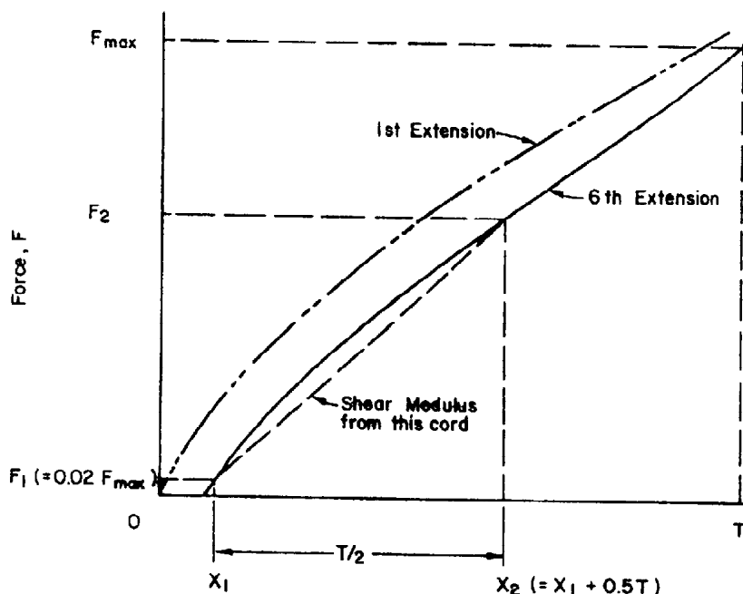
FIG. A1.2 Shear Test Force - Extension Curves
